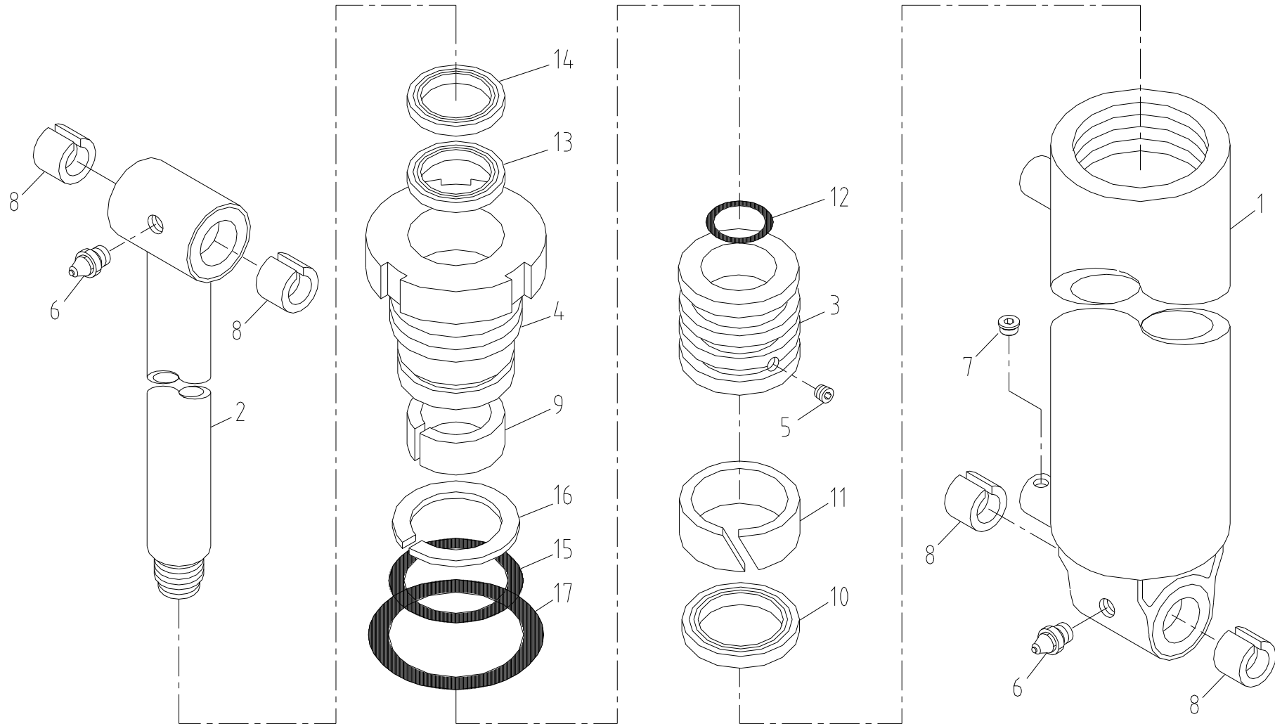
Fig. 2-1 SCS1516 DERRICK CYL' ASS'Y
