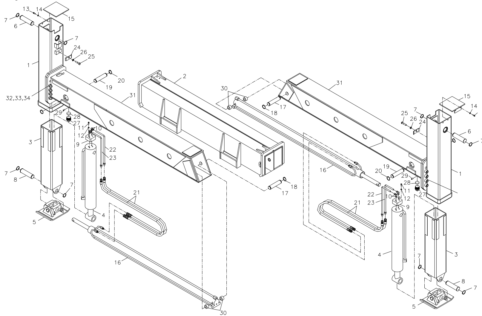
Fig. 9-2-1 SCS1516 REAR OUTRIGGER ASS'Y
