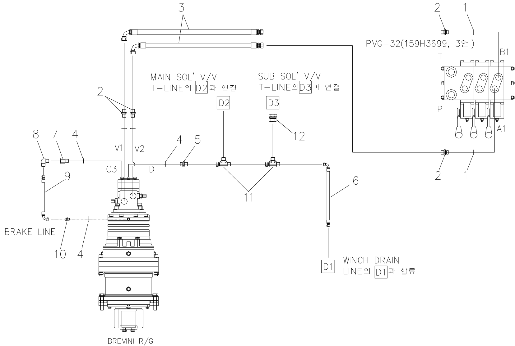
Fig. 5-2 SCS1516 SWING PIPING
