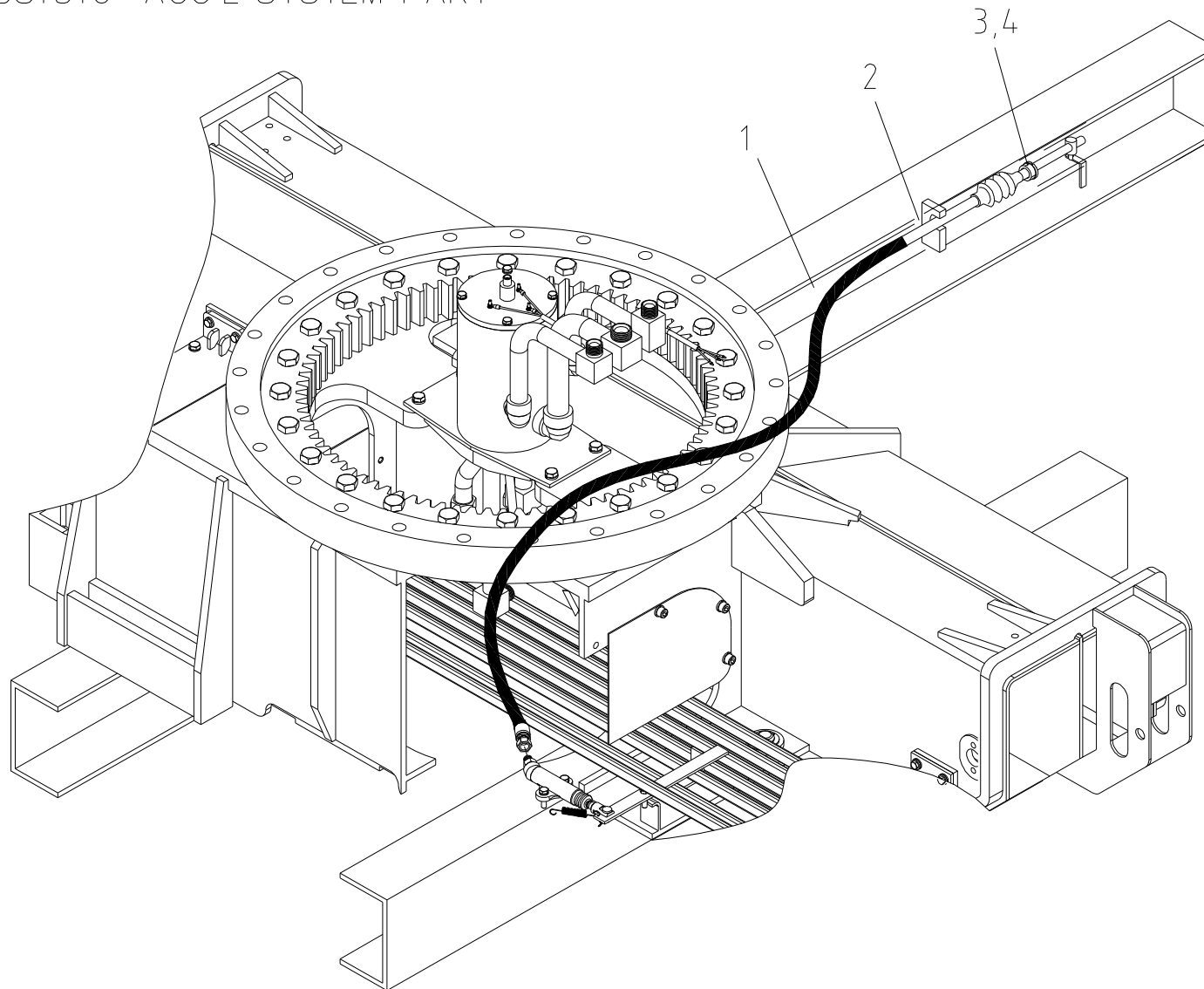
Fig. 9-3 SCS1516 ACC'L SYSTEM PART
