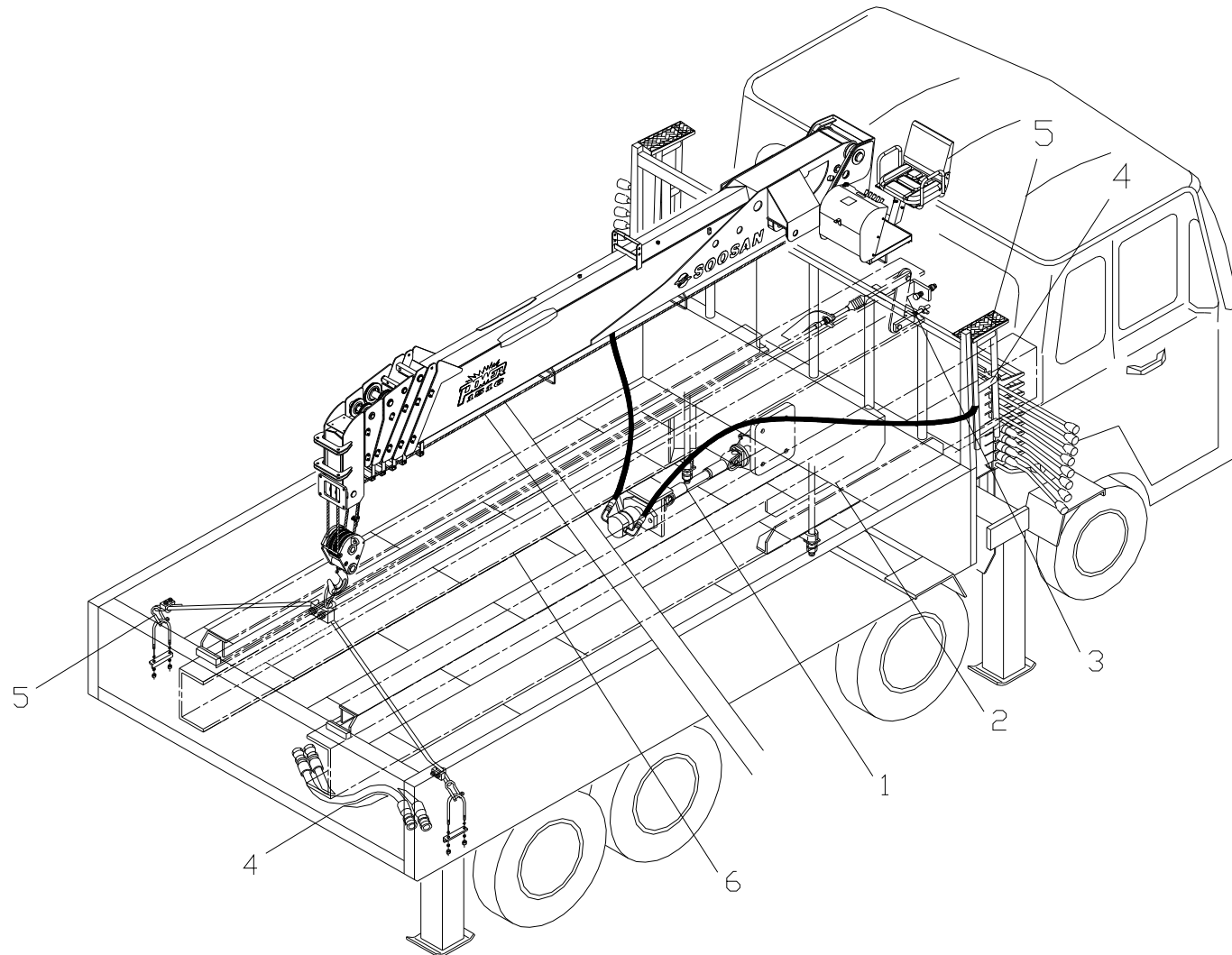
장착조립체 Fig. 9 SCS1516 MOUNTING ASS'Y
