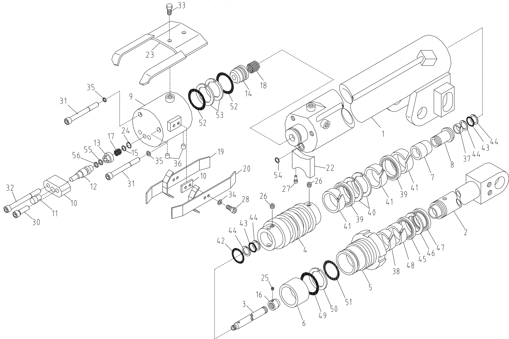
Fig. 1-1-1 SCS1516 TELESCOPIC CYL'(1st) ASS'Y
